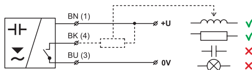
Fig. 7: NPN type sensors connection (version "N")
