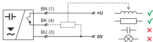
Fig. 9: PNP type sensors connection (version "P")
