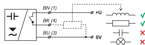
"P" (PNP) type sensors connection
