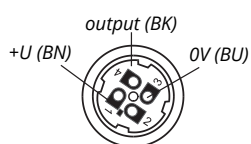
Inside of the connector socket
