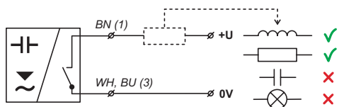
"S" type sensors connection (2 - wire electronic switch)
