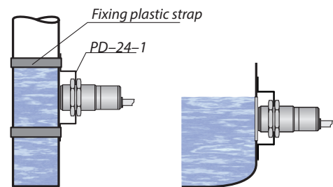
CPS sensor application for level gauges and eye sights
