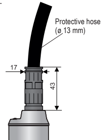
Variant "H" with cable gland for protected hoses - for using in an outdoor area or in area with increased moisture.
