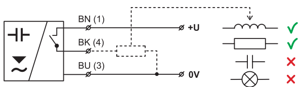
PNP type sensors connection (version "P")
