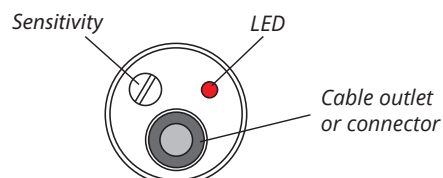
Top view of level sensor
