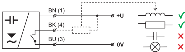
NPN type sensors connection (version "N")
