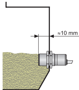
Sensing bulk-solid materials in storage tanks
