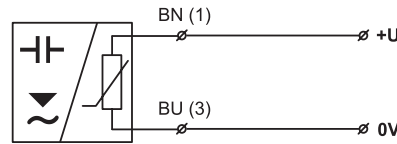
NAMUR type sensors connection (version "Xi")
