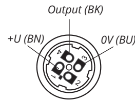
Inside of the connector socket
